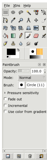
Figura 17.1 Janela principal
